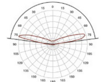
LIGHT DISTRIBUTION GRAPH Beam angle is 175°
