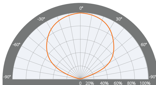
Latitudinal (vertical angle) Polar Radiation Pattern
