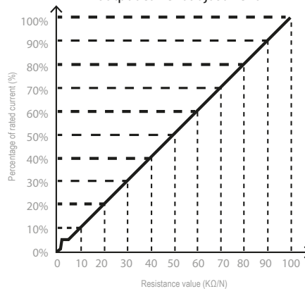
Resistance value for output current adjustment
