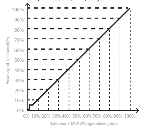
10V PWM signal for output current adjustment, Frequency range: 100Hz-3KHZ
