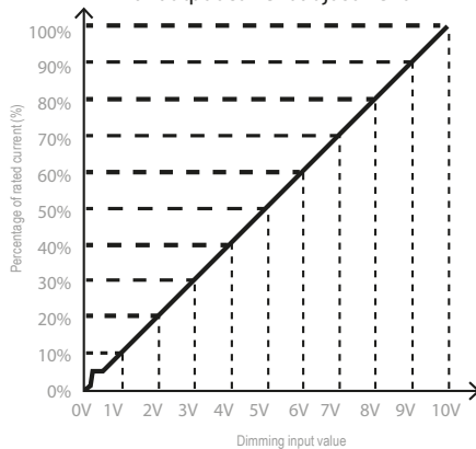
0-10V dimmable function for output current adjustment
